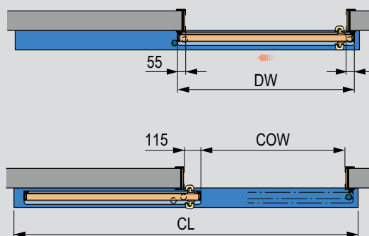
Besam Hermetic-L Left opening shown, right opening mirror image
